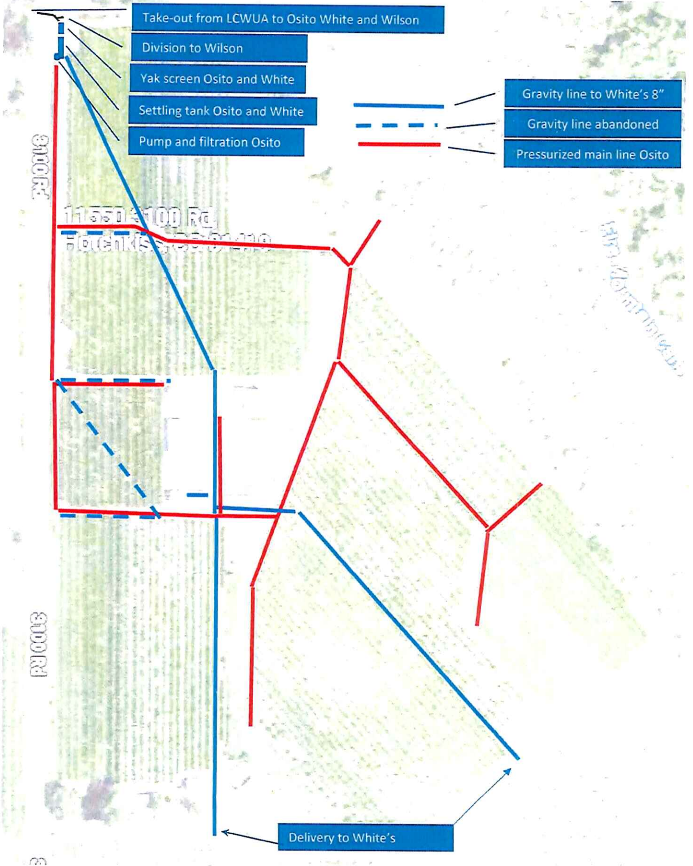
Osito Orchard Irrigation schematic – approximate positions - 2020
